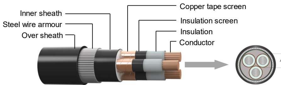
Cable construction
